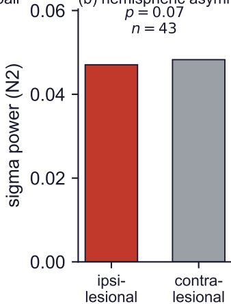
(b) hemispheric asymmetry
