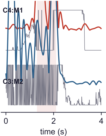
(a) sigma envelope on homologous pair
